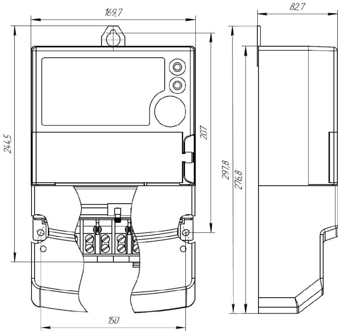
Fig 2.1 – Overall and mounting dimensions of the meter
